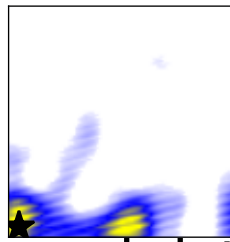
Deterministic prediction
